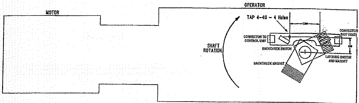
TOP VIEW - DOOR HINGED AT RIGHT
