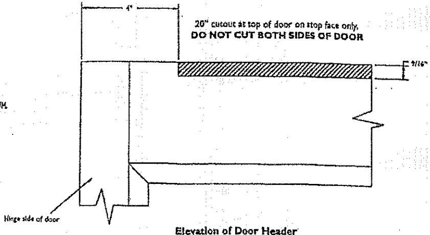
Elevation of Door Header
